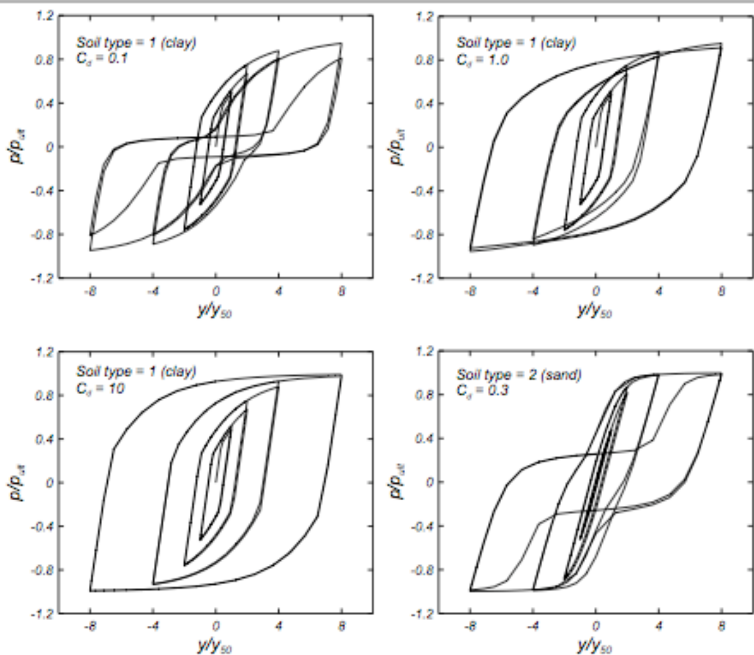
FIG. Four examples of cyclic loading response; three for soilType = 1 with C_d = 0.1 , 1.0, and 10, and one for soilType = 2 with C_d = 0.3 .
